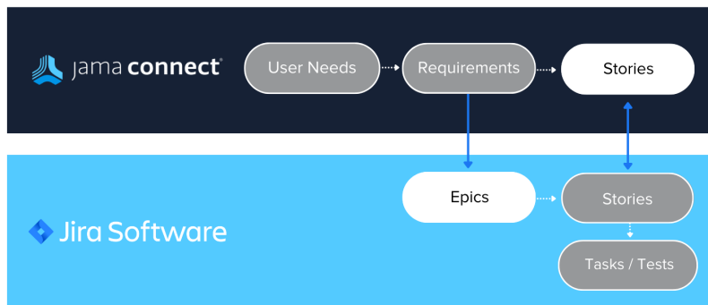
Sample integration between Jama Connect and Jira
